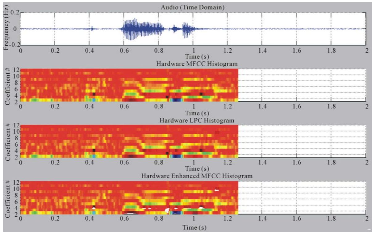
Figure 9. Hardware frontend histograms with audio data (12_Coefficients) (due to limited amount of hardware resources the part of the data is not show in the resulting spectrograms).
