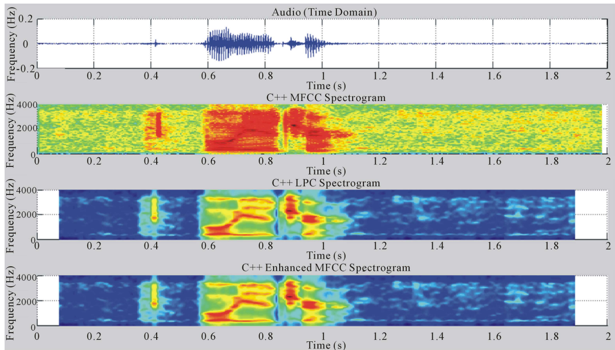
Figure 6. C++ frontend spectrograms with audio data.
