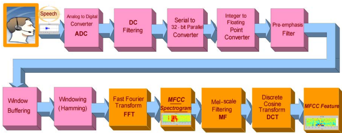
Figure 3. MFCC feature extraction.
