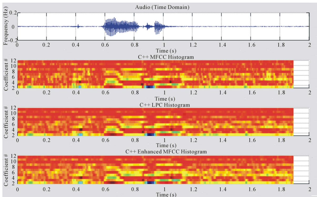
Figure 8. C++ frontend histograms with audio data (12_Coefficients).
