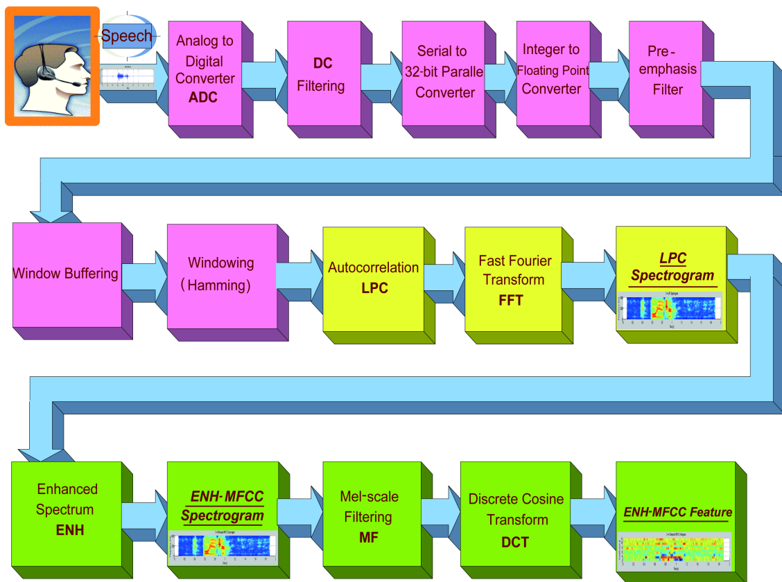
Figure 5. ENH-MFCC feature extraction.
