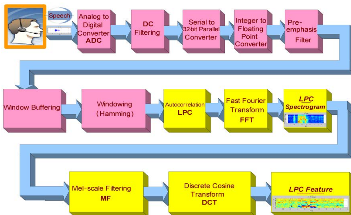
Figure 4. LPC feature extraction.
