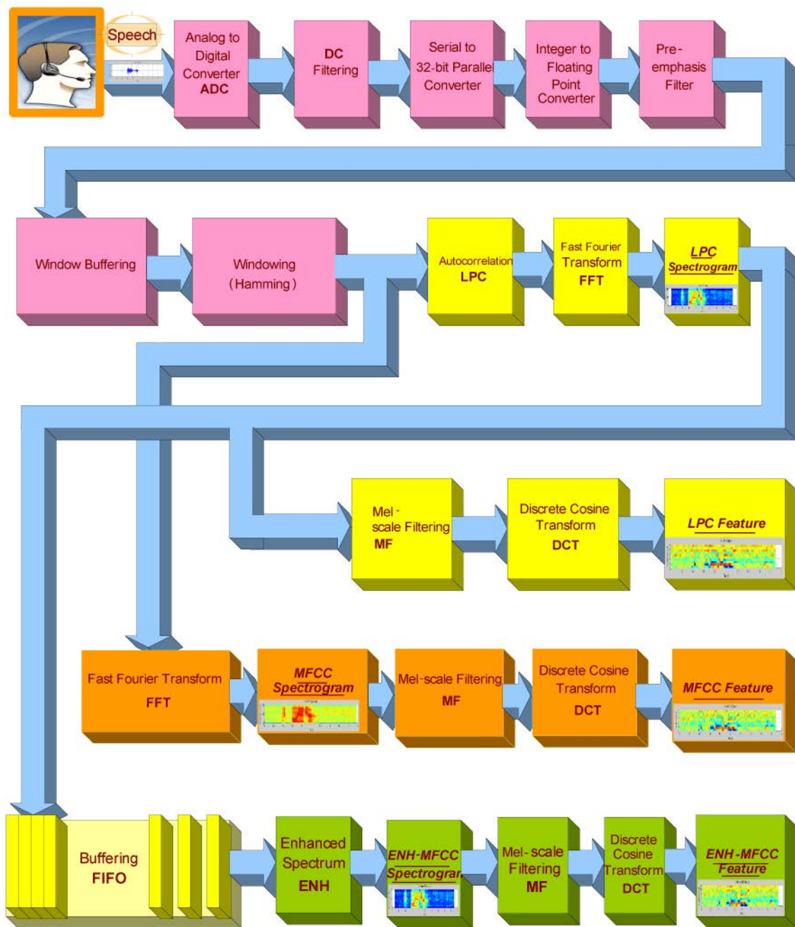
Figure 2. Overall front-end of WUW-SR block diagram.
