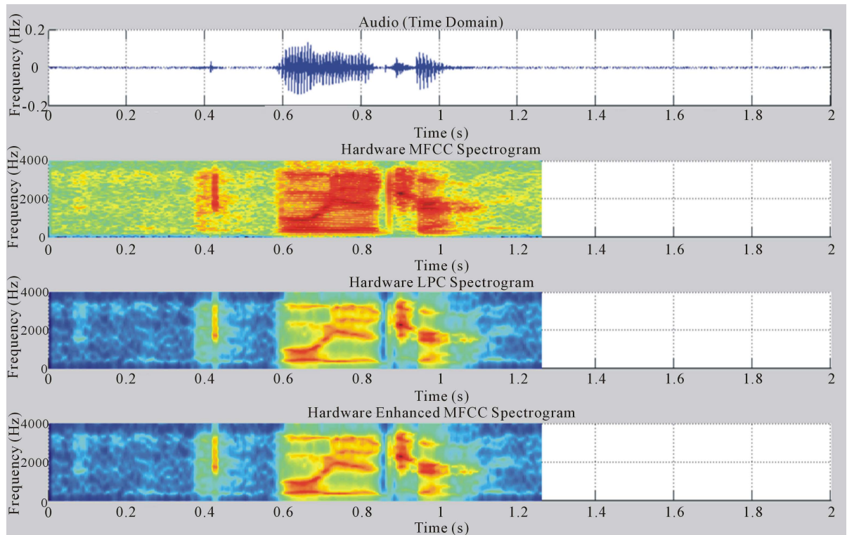
Figure 7. Hardware frontend spectrograms with audio data (due to limited amount of hardware resources the part of the data is not show in the resulting spectrograms).
